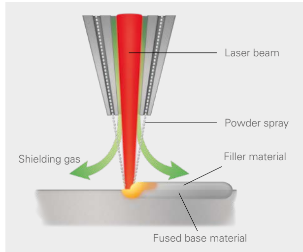
Laser metal deposition with powder (LMD-P)
