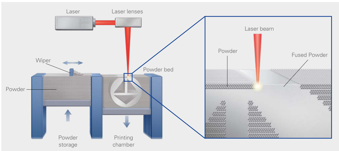
Laser Powder Bed Fusion (L-PBF)
