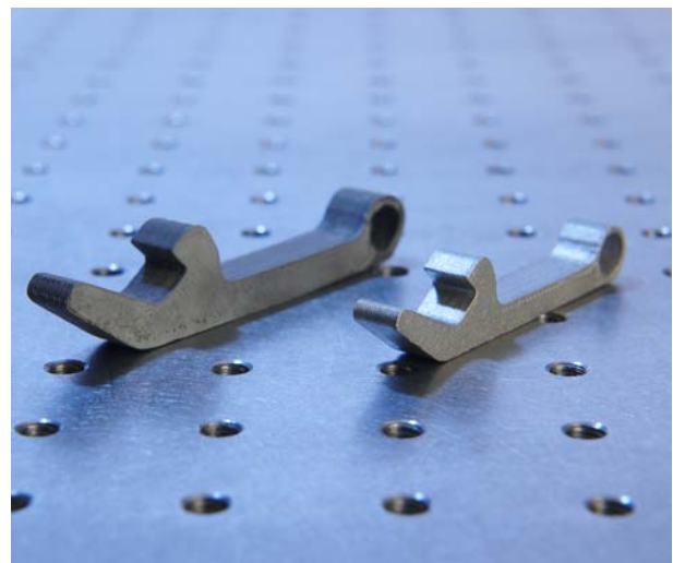
Binder jetting (left: green body, right: finished component)
