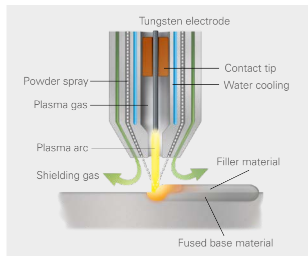
Plasma-arc deposition welding
