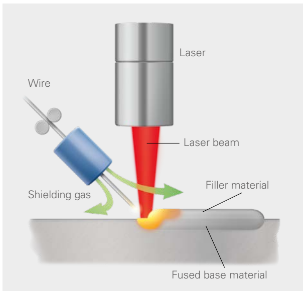
Laser deposition welding with wire (LMD-W)
