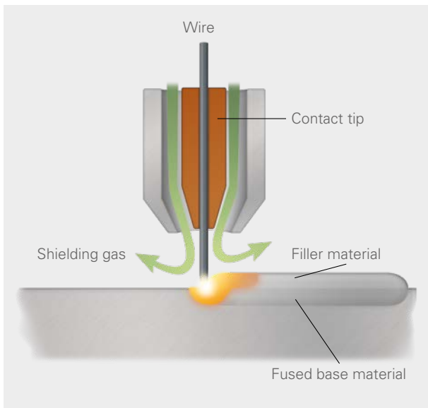
Wire arc additive manufacturing (WAAM)
