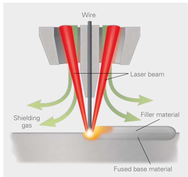
Coaxial laser metal deposition with wire (LMD-W)
