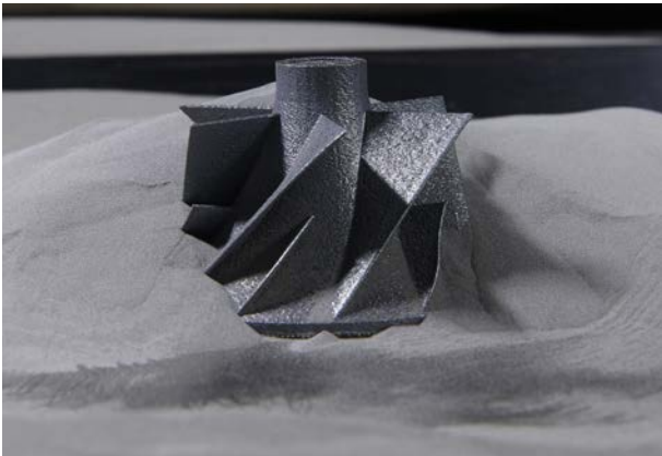
Turbocharger from a powder bed, produced by ifw Jena
